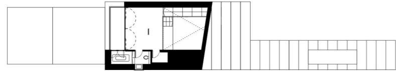
annex first floor
